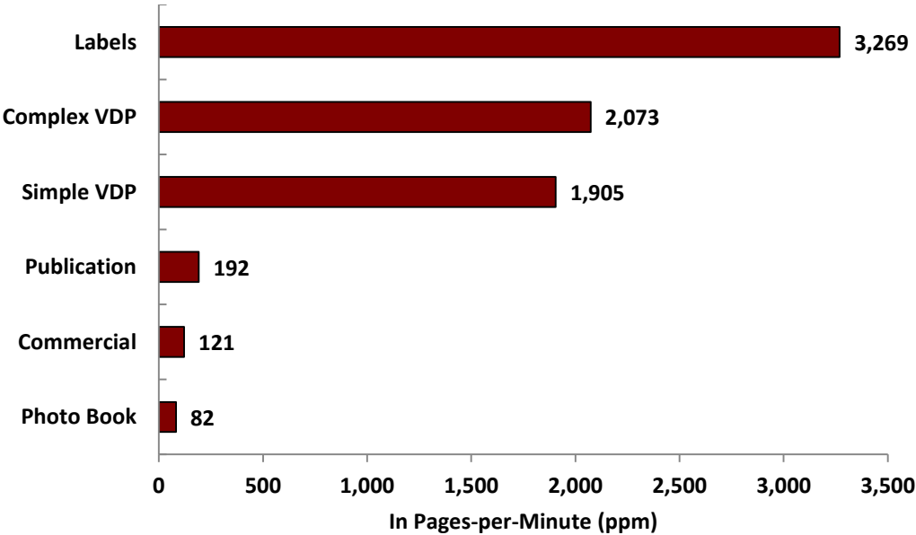
Figure 6: Measured Speeds of a single Harlequin RIP by Category
