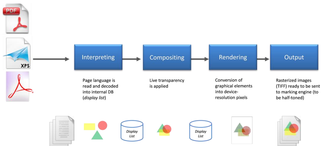
Figure 2: The RIP process explained
